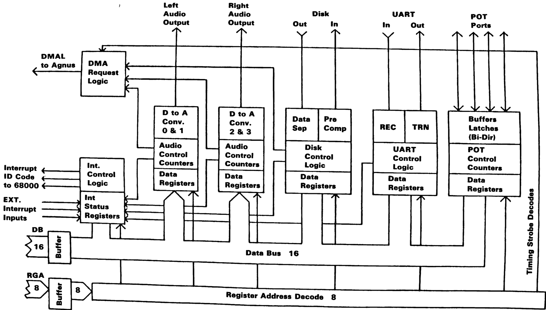
Paula Block Diagram
