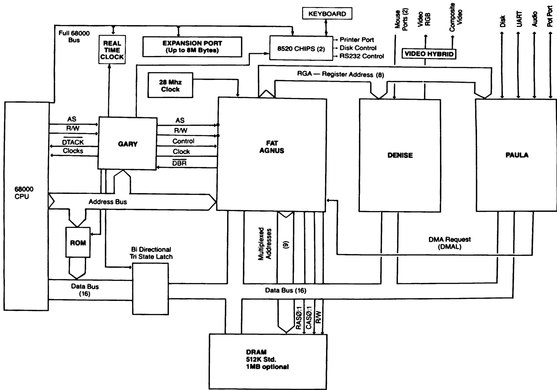
A500 Block Diagram
