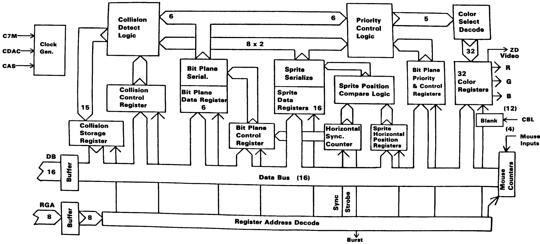
Denise Block Diagram
